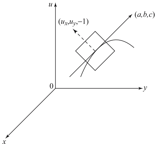
Figure 2.4.1 Tangent and normal vector fields of solution surface at a point (x, y, u) .
