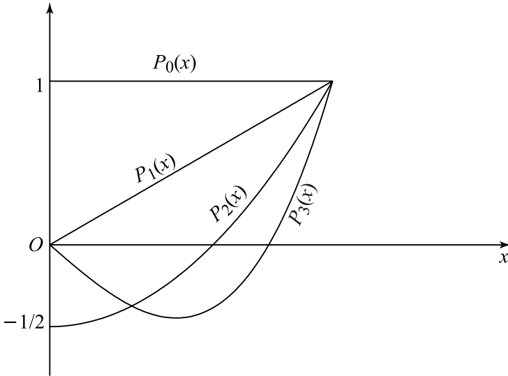
Figure 8.9.1 The first four Legendre's polynomials.
